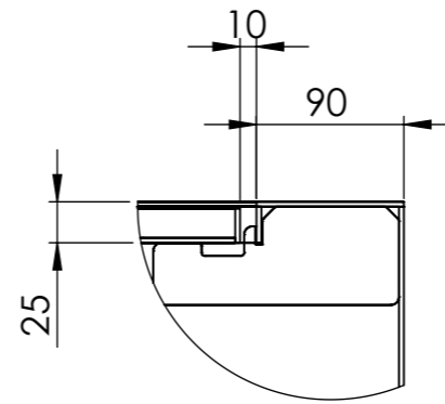
DETAIL D SCALE 1 : 5
